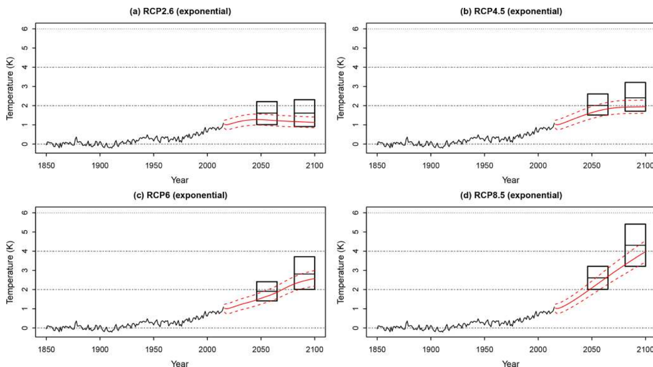
Figure 5. Panels (a)–(d) describe the marginal posterior means and 95 % credible intervals of the predicted temperature response to future forcing according to the RCP2.6, RCP4.5, RCP6, and RCP8.5 trajectories, respectively, using a single-exponential response function. These are compared to the AR5 projections (black boxes).
