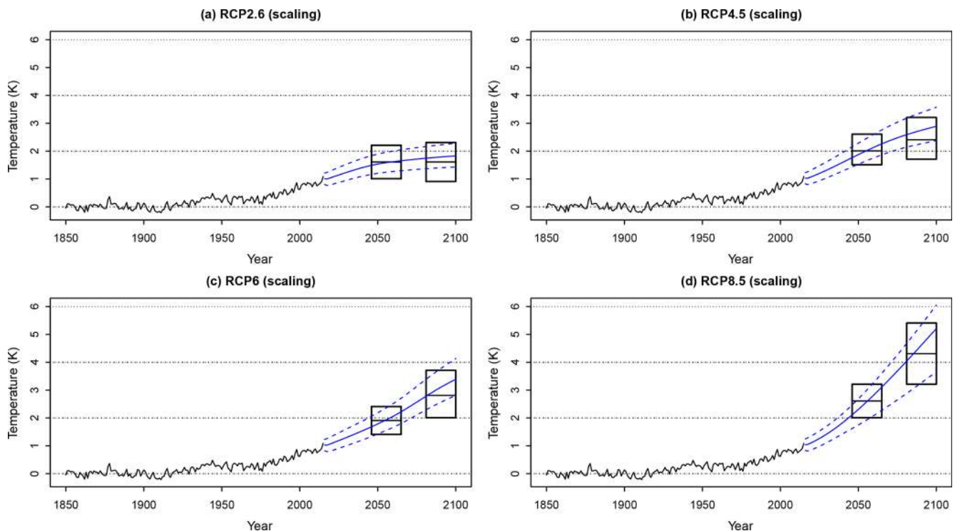
Figure 4. Panels (a)–(d) describe the marginal posterior means and 95 % credible intervals of the predicted temperature response to future forcing according to the RCP2.6, RCP4.5, RCP6, and RCP8.5 trajectories, respectively, using a scaling response function. These are compared to the AR5 projections (black boxes).
