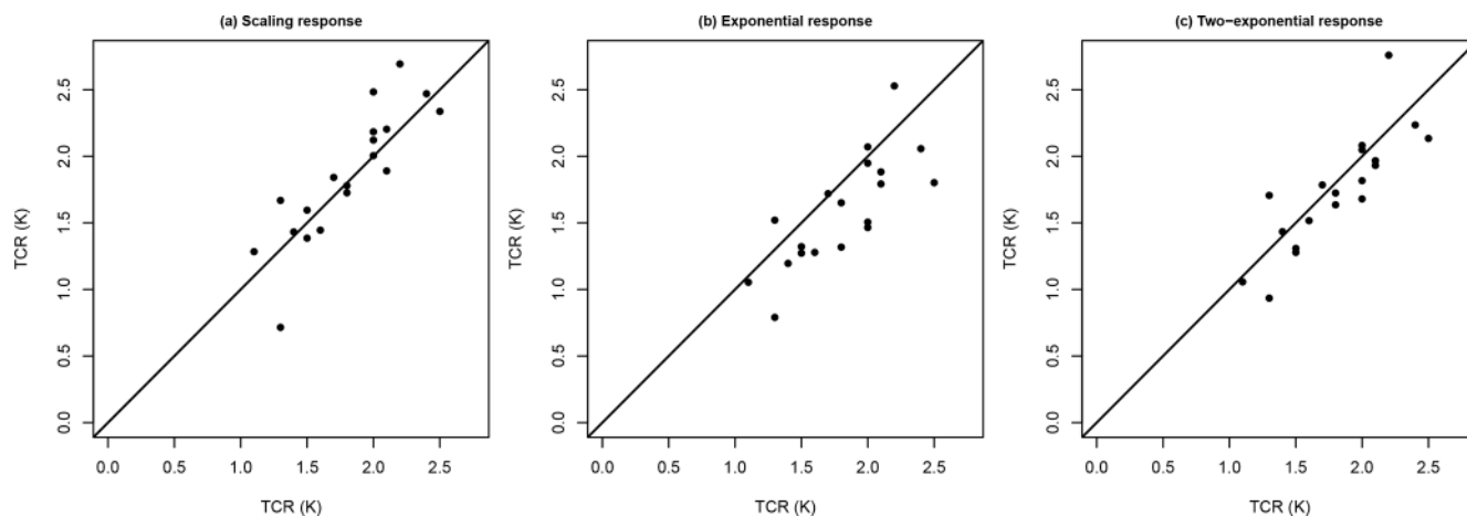
Figure 8. Scatter plot of the TCR obtained directly from the 19 ESMs against the corresponding marginal posterior mean estimates when using a scale-invariant response function (a), a single-exponential response function (b), and a two-exponential response function (c).
