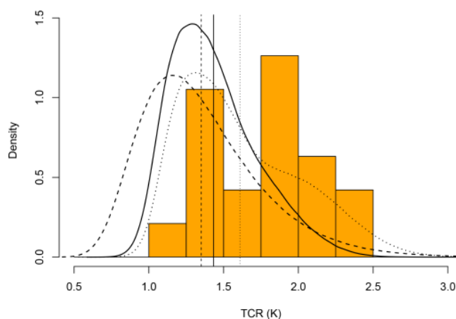
Figure 10. Histogram of the TCR obtained from the different ESMs with the posterior density function estimated from the Monte Carlo simulations using a scale-invariant (solid), a single-exponential (dashed), and a two-exponential (dotted) response function. The vertical lines describe the means of the three approaches.
